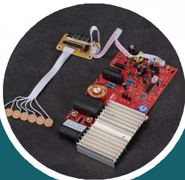
Induction cook top
